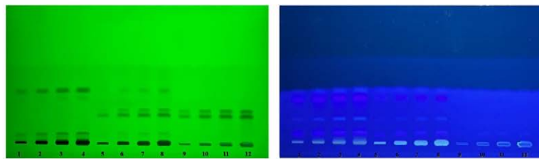
HPTLC profile in water, mobile phase Toluene: Ethyl acetate: Formic acid (5:4:1) (M2). From 1 to 12: Track 1-4: pure extract, Track 5-8 :granules(JMBG), Track 9-12:excipients in UV 254 nm(Green) and UV 366 nm (Blue)
