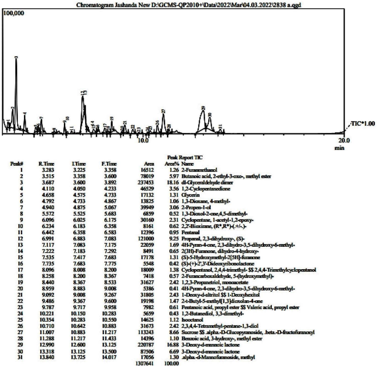
Figure 4: GCMS graph with NIST - Peak Report TIC of Joshanda (JMB).
